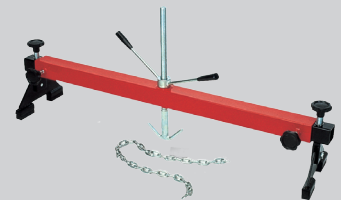
Model 583 Transverse Engine Support
